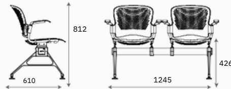
VENUS GANG CHAIR 3 SEATER WITH HANDLE - ( L / W / H : 1890 / 610 / 812 )
